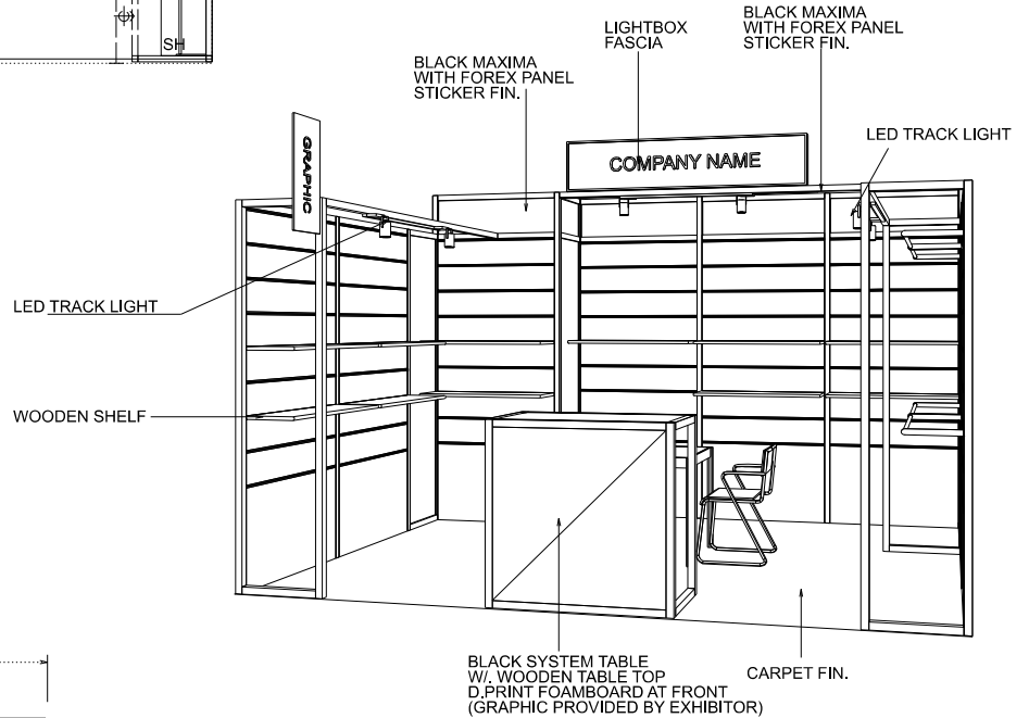
PERSPECTIVE
